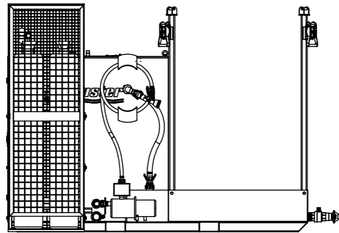
MOBILE CONCRETE WASHOUT (MCW)
