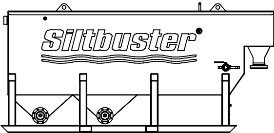
CM400 OWS L: 3705mm W: 1200mm H: 1750mm
