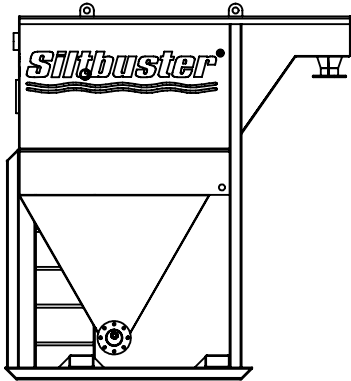
HB20 OWS L: 2284mm W: 1430mm H: 2485mm
