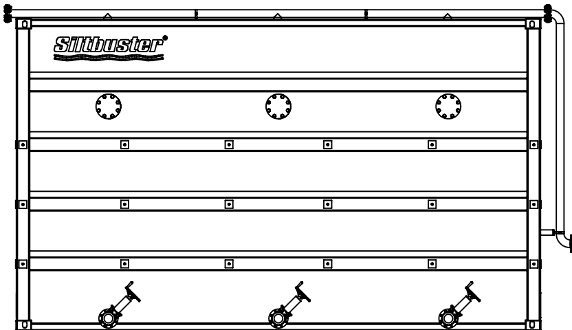
MBBR30 L: 6060mm W: 2440mm H: 3755mm
