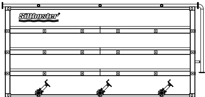
MBBR20 L: 6060mm W: 2440mm H: 3025mm
