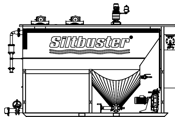
IHB20R L: 4184mm W: 1490mm H: 2970mm H: 2420mm (BRIM)
