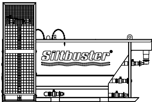
HYDRODEMOLITION UNIT L: 2749mm W: 1331mm H: 1824mm H: 1148mm (BRIM)
