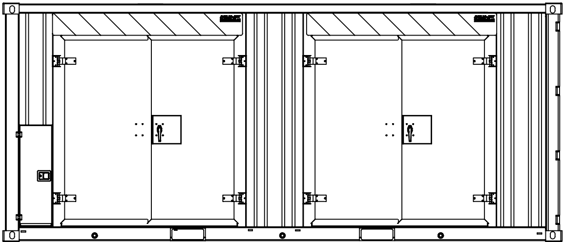
ECOCLEAR 2.0 L: 6060mm W: 2440mm H: 2590mm
